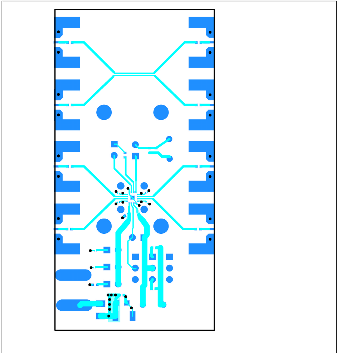
Figure 4. MAX3748 EV Kit PC Board Layout – Component Side (2X)
