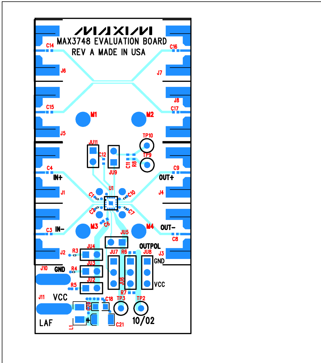
Figure 3. MAX3748 EV Kit Component Placement Guide – Component Side (2X)
