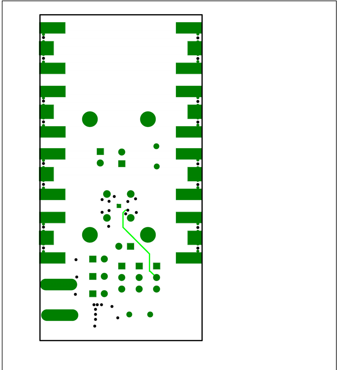
Figure 7. MAX3748 EV Kit PC Board Layout – Solder Side (2X)
