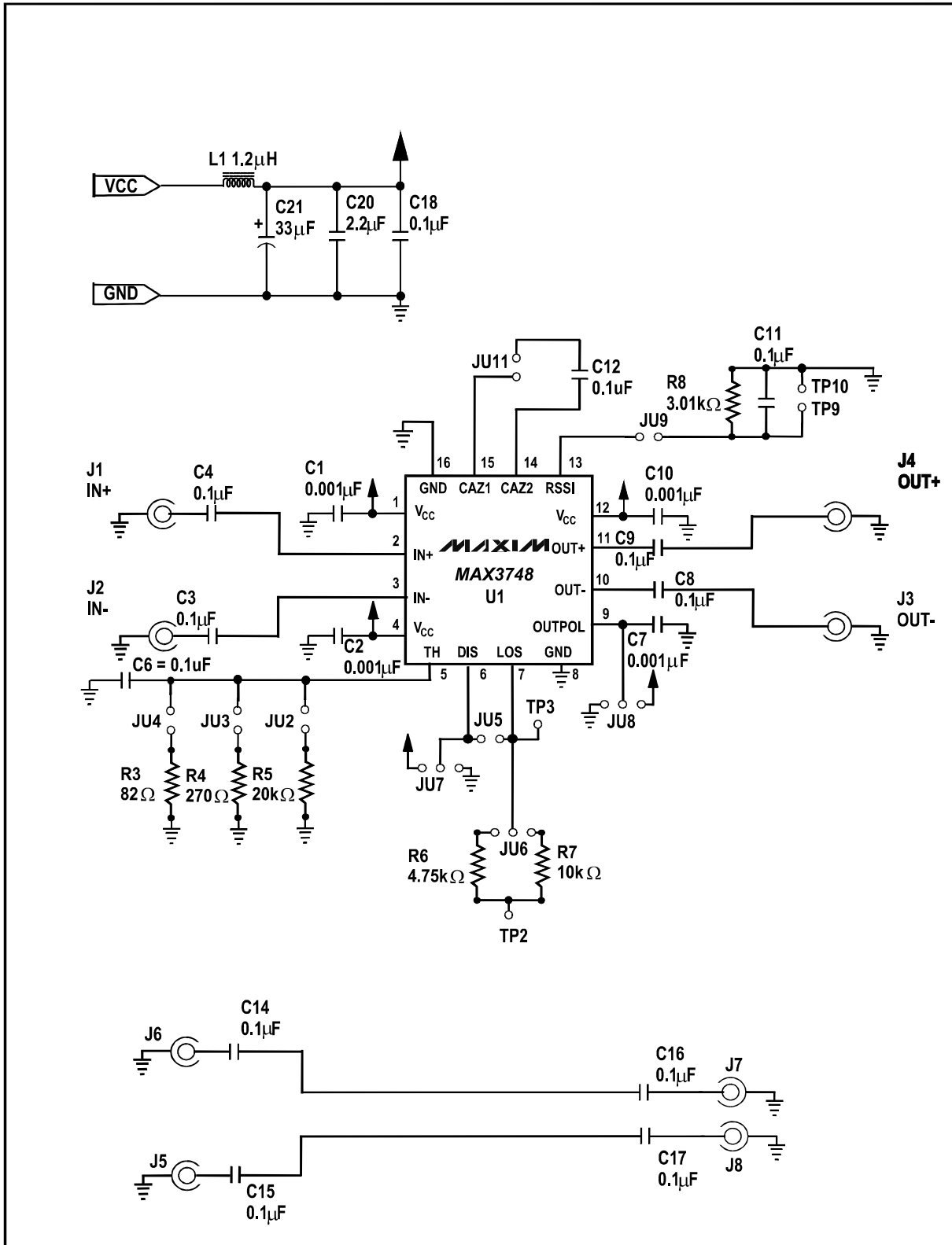
Figure 1 MAX3748 EV Kit Schematic.
