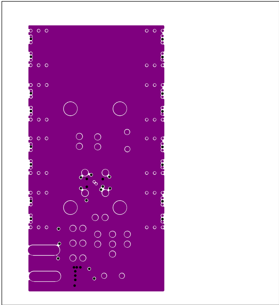
Figure 6. MAX3748 EV Kit PC Board Layout – Power Plane (2X)
