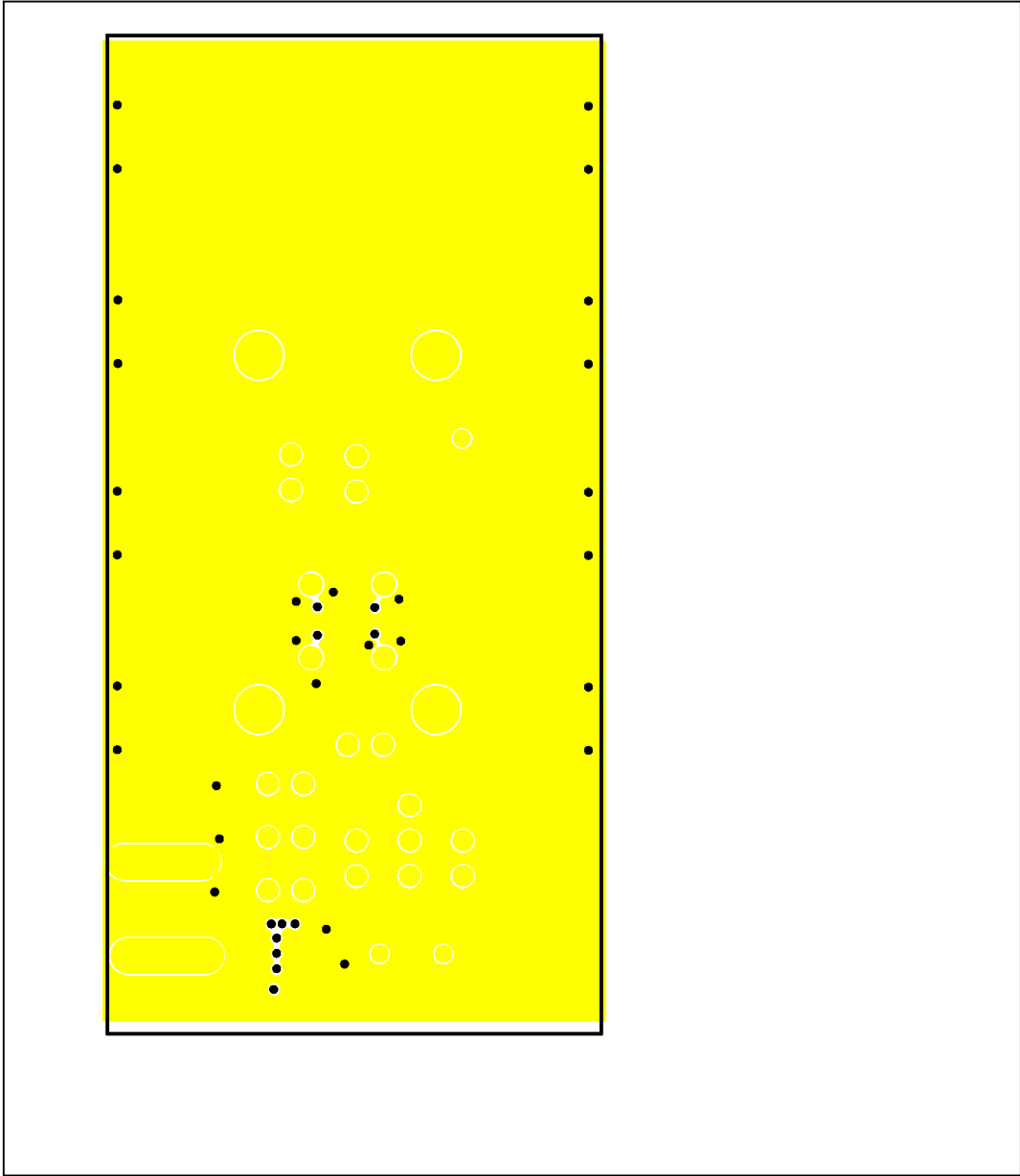
Figure 5. MAX3748 EV Kit PC Board Layout – Ground Plane (2X)
